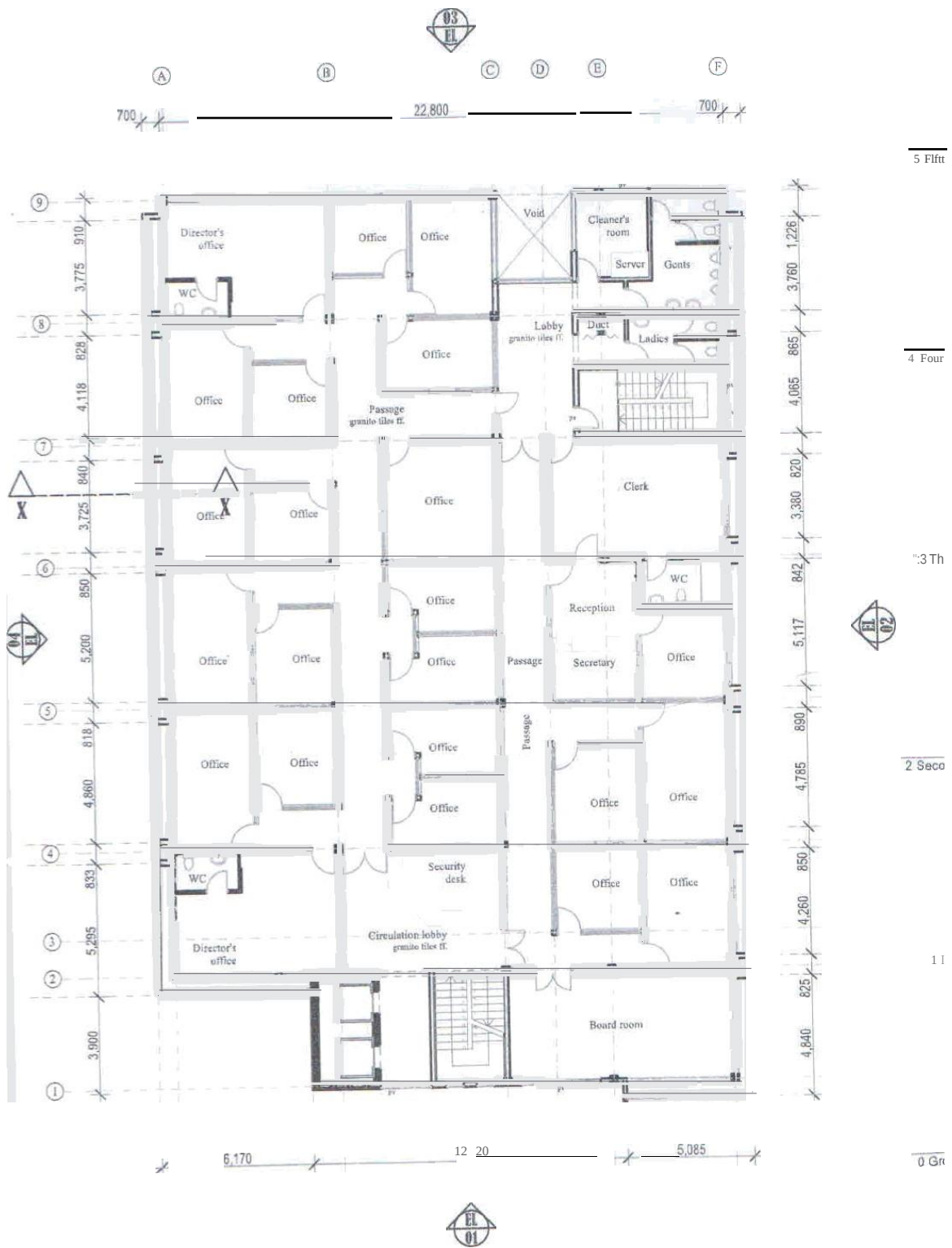
TYPICAL FLOOR PLAN LAYOUT
