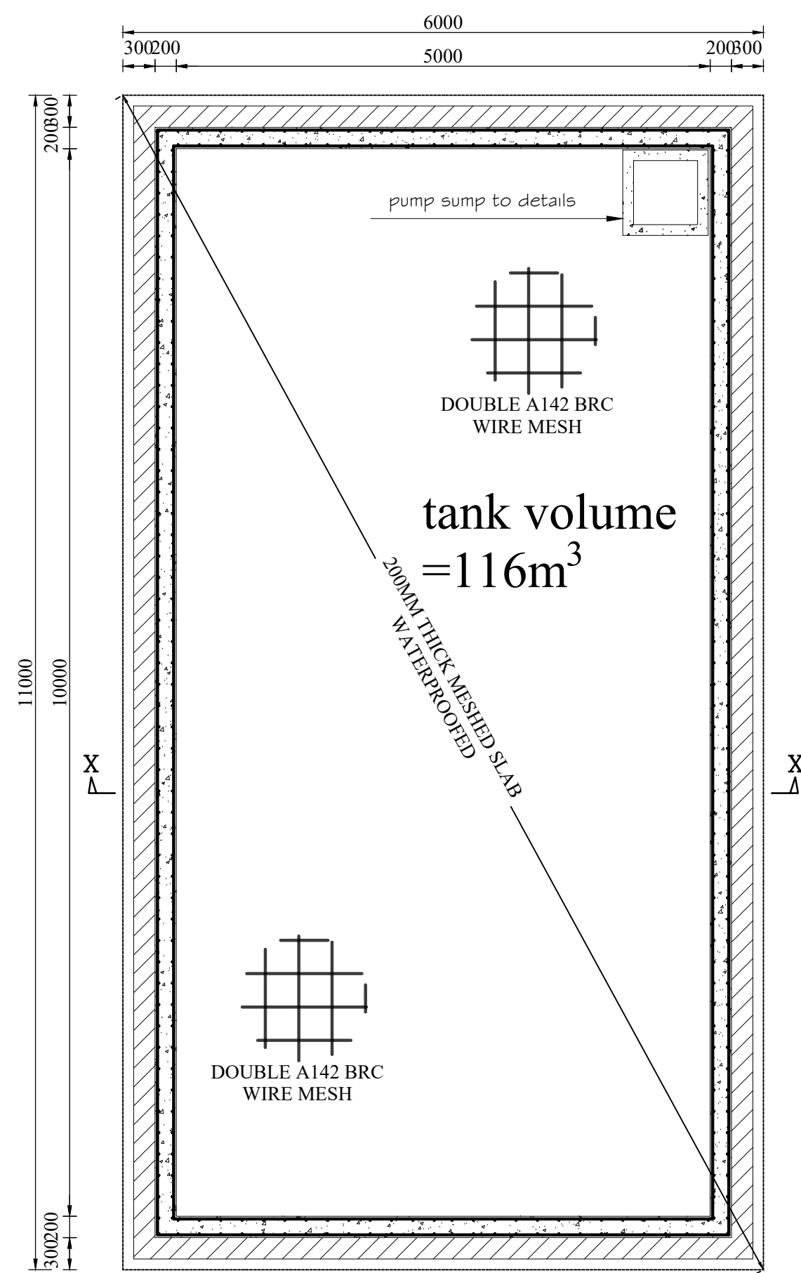
FOUNDATION LAYOUT SCALE 1:50
