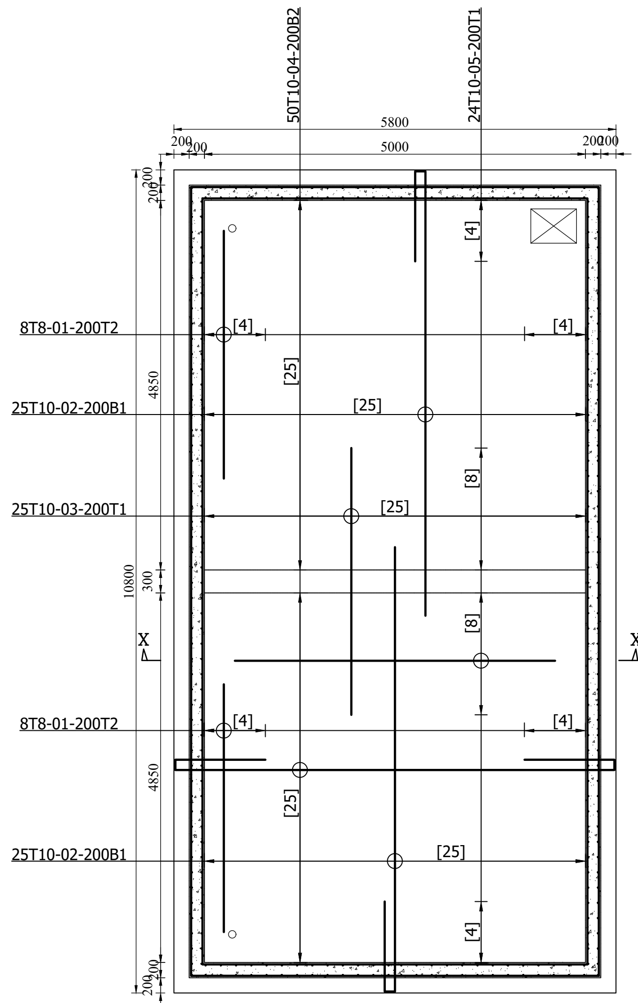
SLAB DETAILS SCALE 1:50
