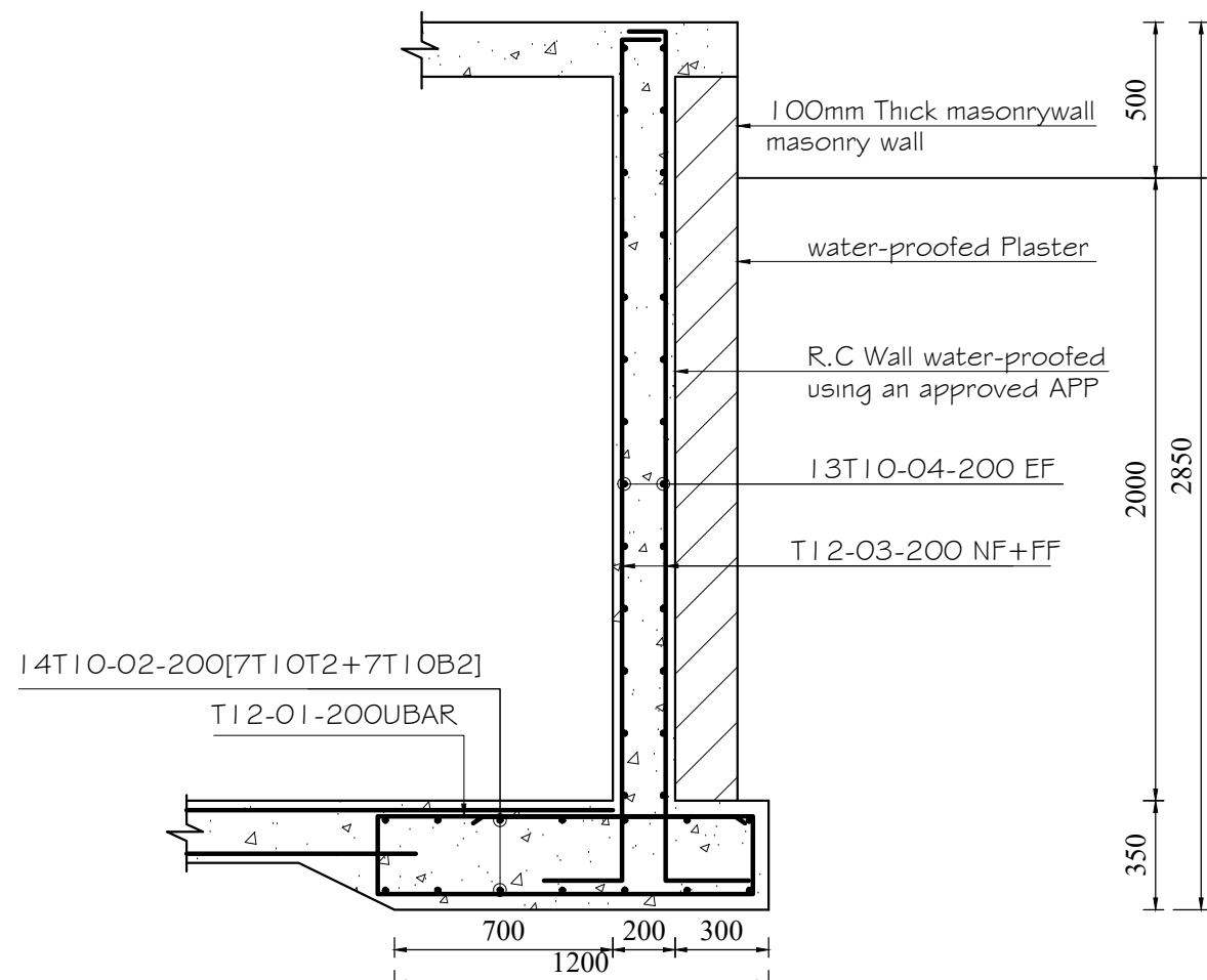
R.C RETAINING WALL SECTION FOR WATER TANK SCALE 1:25
